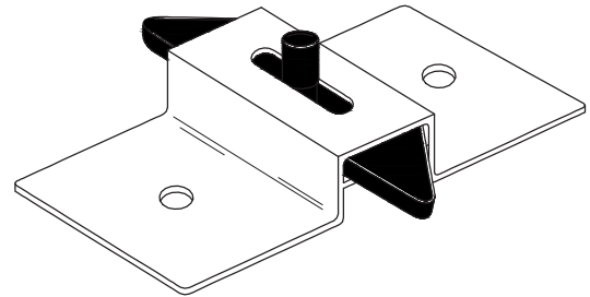
Mitered Latch allows for emergency access (1" Slide Distance)
